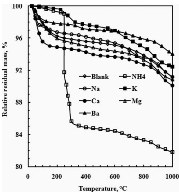
Figure 1. TG plots of ion exchanged vermiculites.
