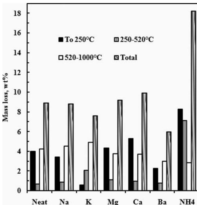
Figure 2. Mass loss of ion exchanged vermiculites.
