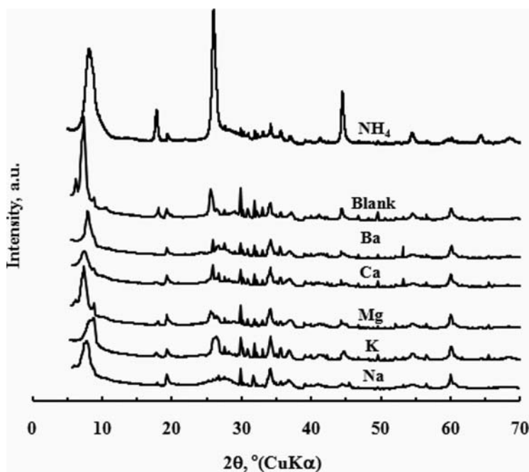
Figure 4. XRD patterns of blank, alkali metal and alkaline metal treated vermiculites.
