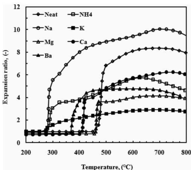
Figure 3. TMA expansion of ion exchanged vermiculites.
