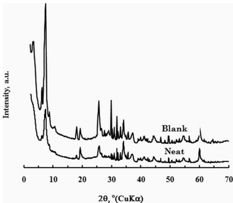
Figure 5. XRD patterns of neat vermiculite and blank vermiculite.
