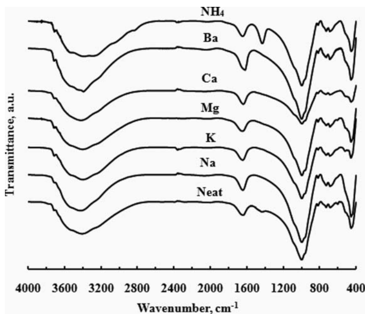
Figure 6. FT-IR spectra of neat vermiculite, ammonium, alkali metal and alkaline metal ion exchanged vermiculites.
